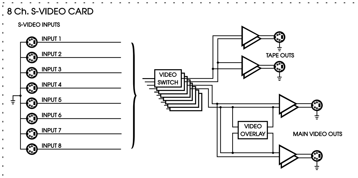
Figure 2a - Block Diagram of 8 S-Video Switching Card
