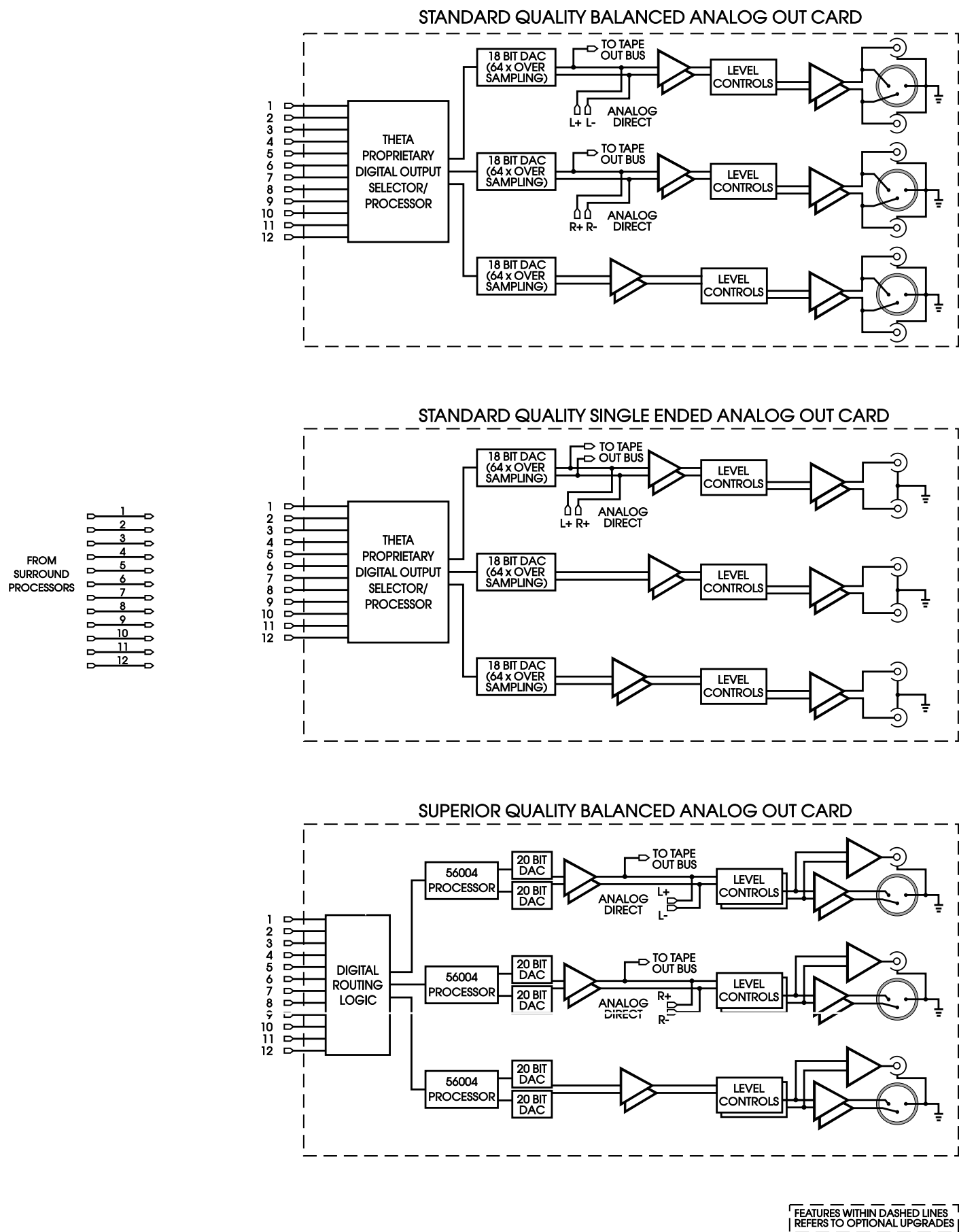
Figure 3 - Block Diagram of DAC and Analog Outputs
