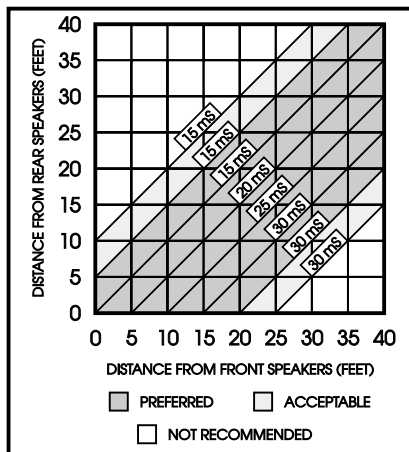
Figure 37 - Rear Delay Settings
