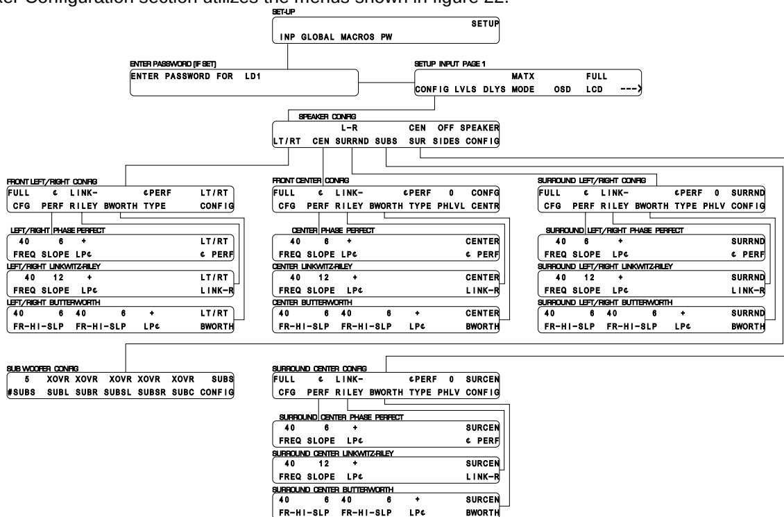
Figure 22 - Menu Map of SETUP/INP Page 1/CONFIG
