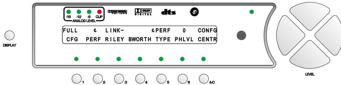
Figure 30 - Front Panel Display of the SETUP/INP/CONFIG/CENTER Sub Menu
